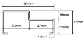
Standard frame profile.
