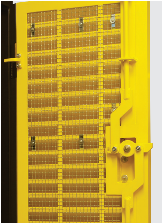
ExcluLouvre® Door 3 incorporating hook bolt system and anti-vermin mesh to rear of frame.
