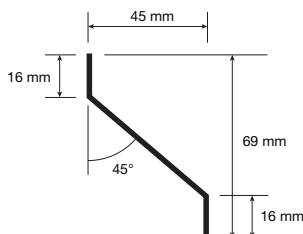
Blade profile
