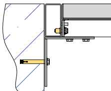
Flanged and non-flanged fixing details.
