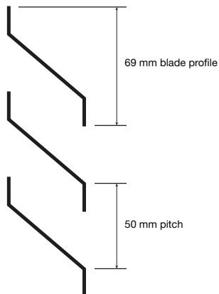
Blade profile and pitch.
