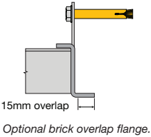
Standard brick fixing
