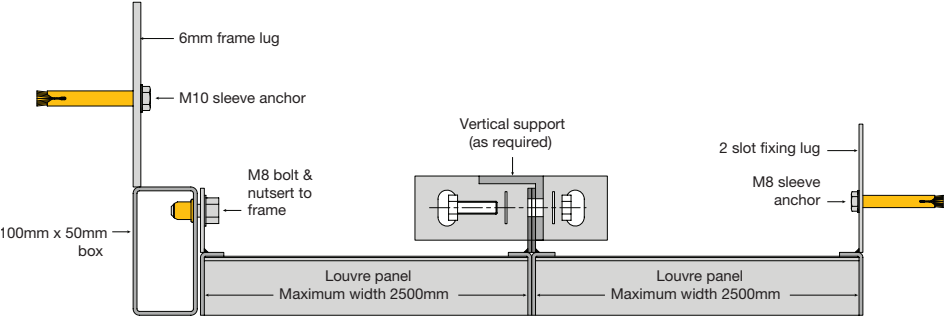
Box frame fixing option.
